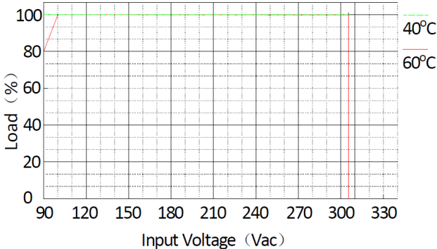
© Input Voltage vs. Load Curve
