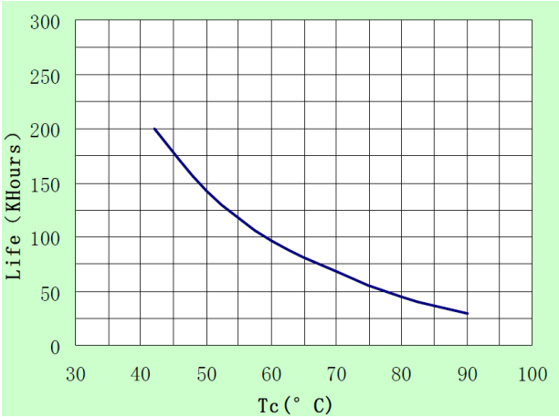
© Life time vs. T_c curve
